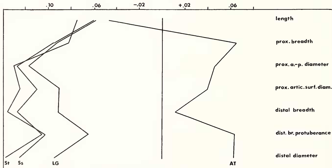
TEXT-FIG. 4. Ratiodiagram (Simpson 1941) comparing MT III of Sinohippus from Altan Teeli (AT), Anchitherium from Steinheim (St), Sansan (Ss), and La Grieve (LG) with Hypohippus (standard) from the Lower Clarendonian of Cherry County, Nebraska.
